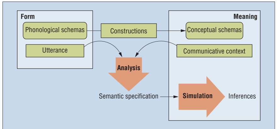
Figure 1. Overview of the Embodied Construction Grammar architecture with two core processes, analysis and simulation. 2
