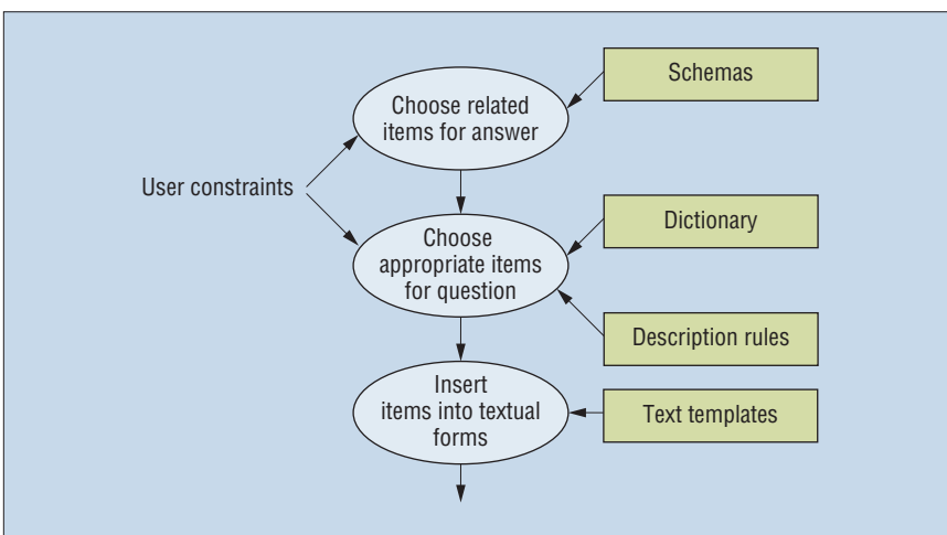
Figure 4. The structure of the STANDUP back end.
