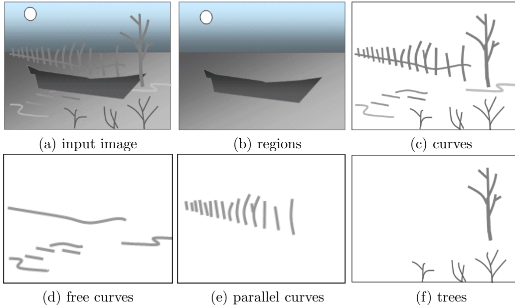
Figure 1: An illustration of parsing an image into regions, curves, and curve groups. (a) is an input image which is decomposed into two layers – (b) a layer of regions and (c) a layer of curves. These curves are further divided into (d) free curves, (e) a parallel curve group for the fence, and (f) trees. Curves observe a partial order occlusion relation.
