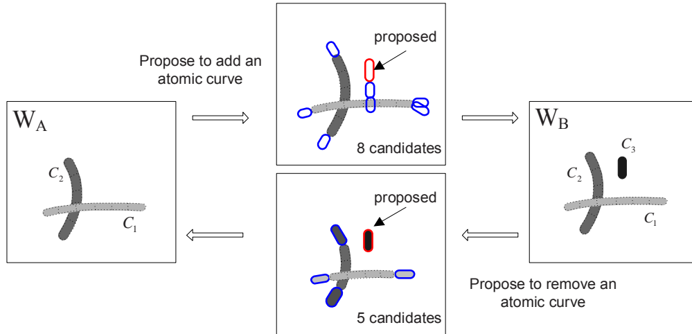
Figure 8: An example of the birth and death of a curve. At state W_A , there are 8 possible atomic curves to be proposed, which are shown as ellipses in the upper middle figure. W_B is the state after selecting an atomic curve to be a new curve. From W_B to W_A , there are 5 candidate atomic curves to be removed, which are shown in the lower middle figure. Choosing the same atomic curve changes W_B back to W_A .
