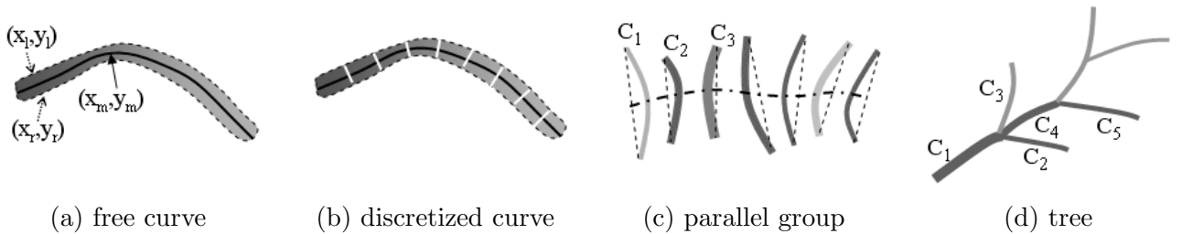
Figure 3: Representations of curves and curve groups. (a) A free curve in continuous representation. (b) A free curve is discretized into a chain of “bars”. (c) Curves for a parallel group (d) Curves for a Markov tree.
